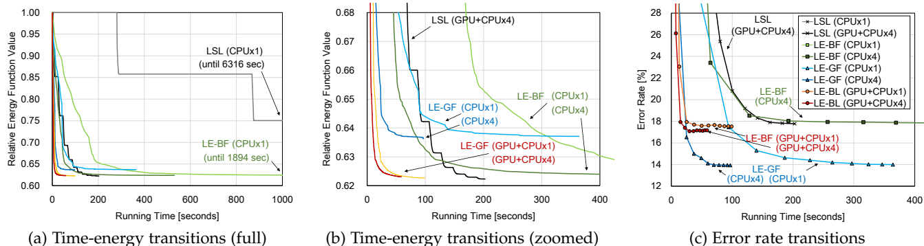
Fig. 9. Efficiency evaluation in comparison to our previous algorithm (LSL) [39]. Accuracies are evaluated for all-regions at each iteration.
