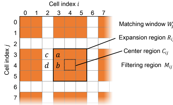
Fig. 5. Expansion regions of mutually disjoint \alpha_{ij} -expansions (group index k = 0 ). We leave white gaps between neighbors.
