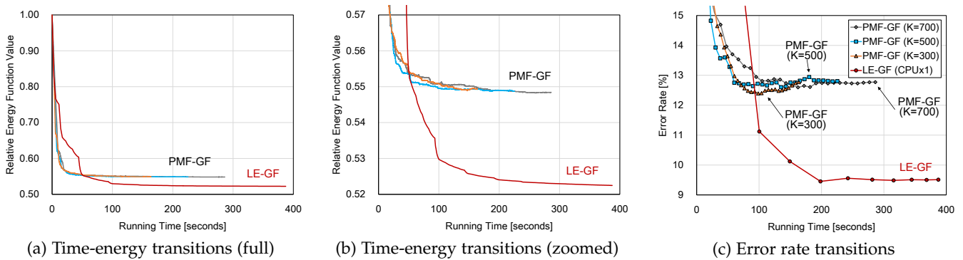
Fig. 12. Efficiency and accuracy comparison with PMF [32]. Our method stably improves the solution and reaches a lower energy with greater accuracy at the convergence. Accuracies are evaluated for all-regions at each iteration. See also Fig. 13 for visual comparison.
