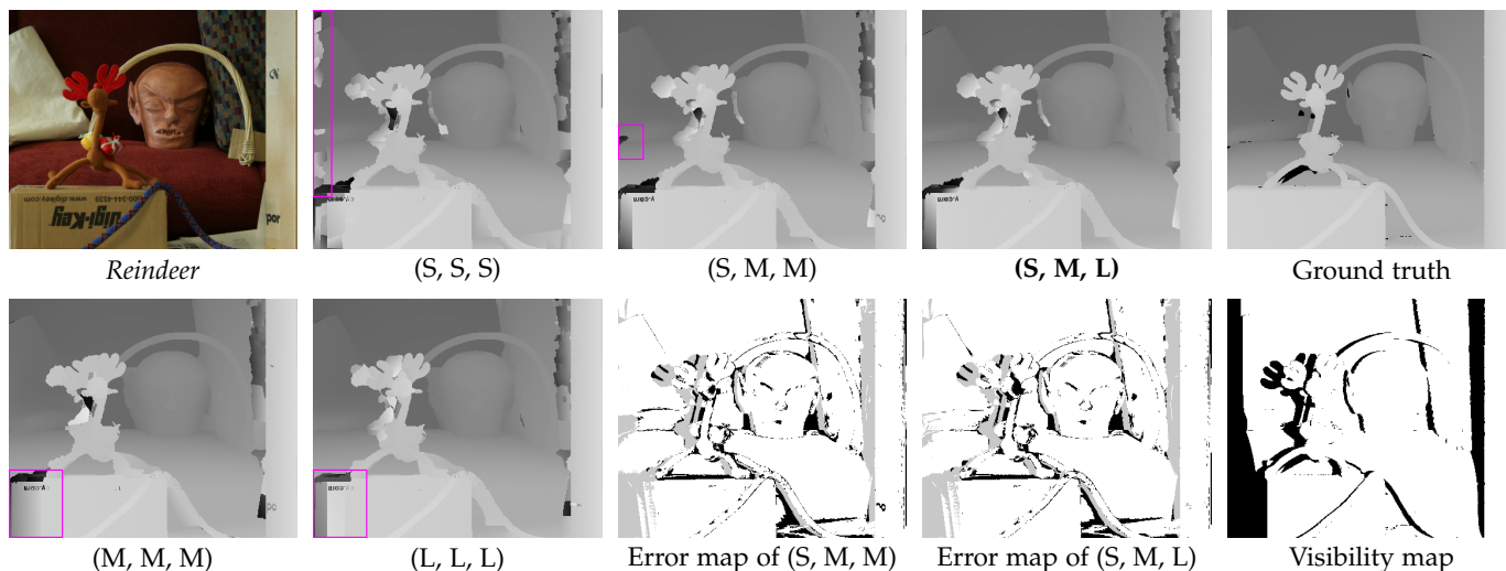
Fig. 8. Visual effect of grid-cell sizes. The use of larger grid-cells leads to smoother solutions and effective for occluded regions. The proposed combination (S, M, L) well balances localization and spatial propagation and performs best. These are all raw results without post-processing.
